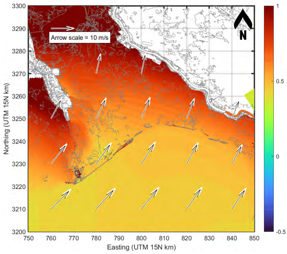
Figure B-13. Instantaneous water level for Scenario 5 (Borrow Pit 1 in NW-SE orientation and Borrow Pit 2) along with wind vectors at 6 p.m. on October 26 th , 2015 (same moment in time as Figure B-12), during the passing of a cold front. The wind-driven water level set-up in the Barataria basin started to decrease compared to Figure B-11.
