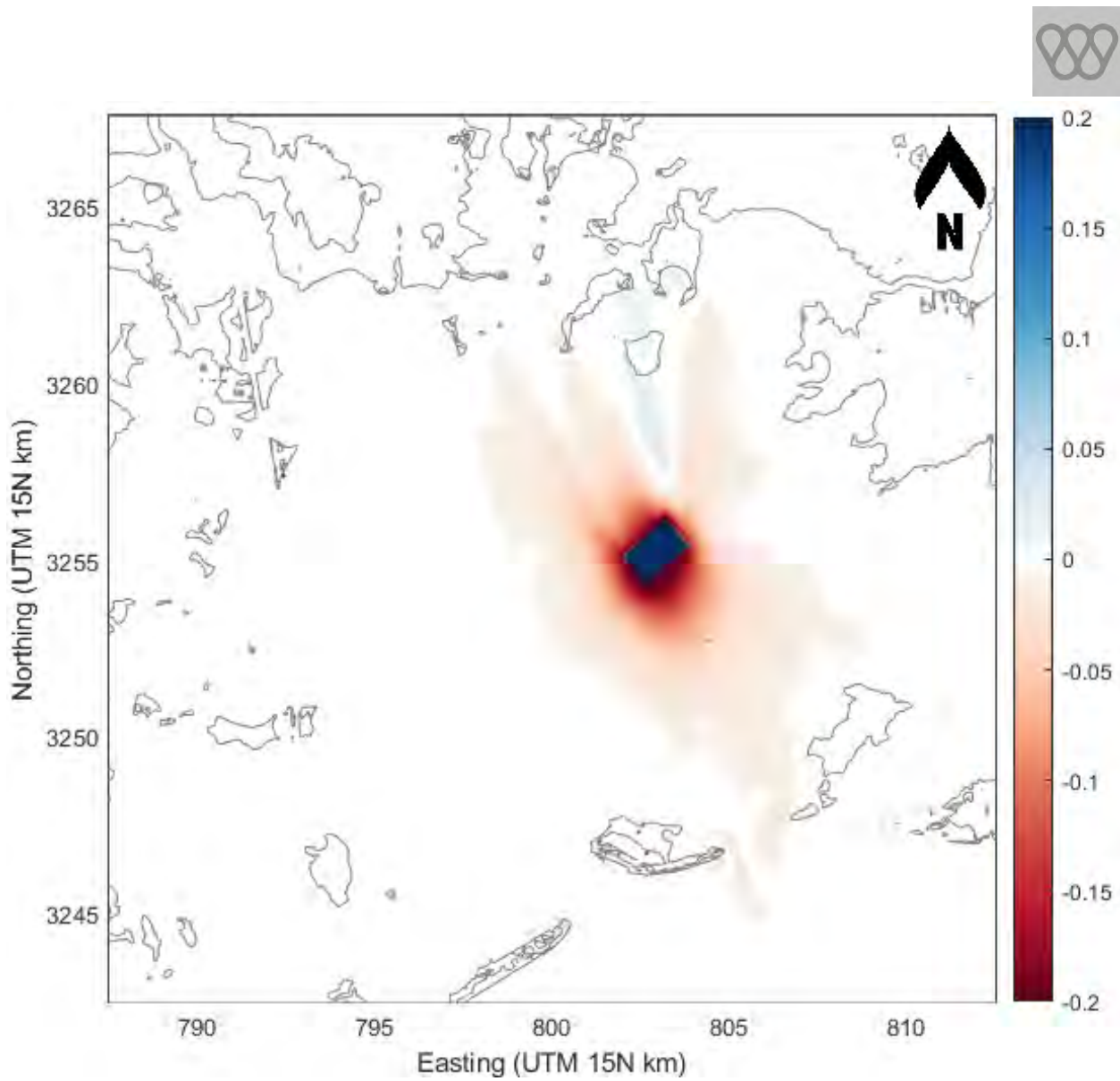
Figure B-23. Modeled bed level change (m) at Barataria Bay differenced to FWOA for S4 (BP2) after 20 years.
