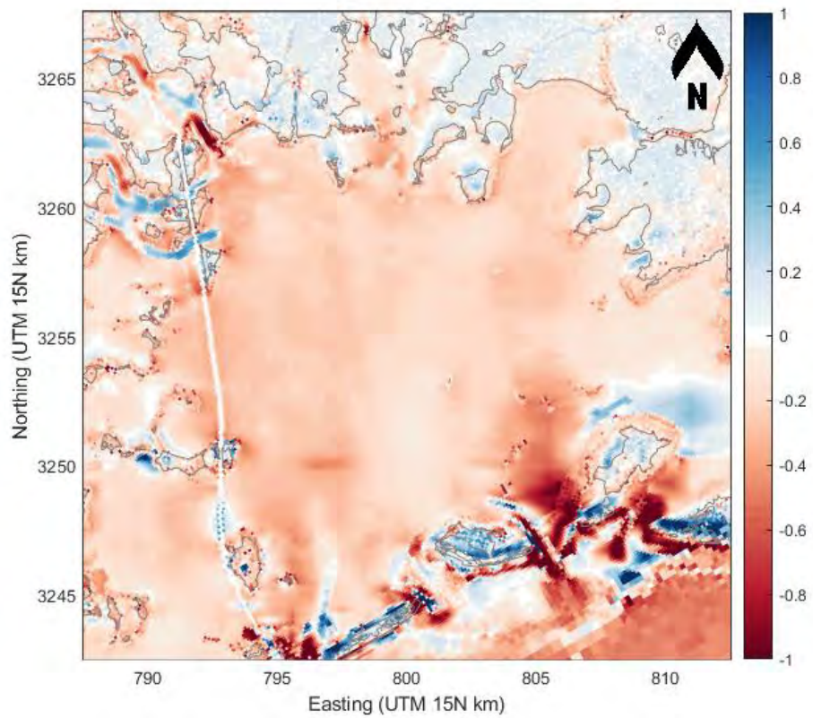
Figure B-16. Modeled bed level change (m) at Barataria Bay for S1 (FWOA) after 20 years.
