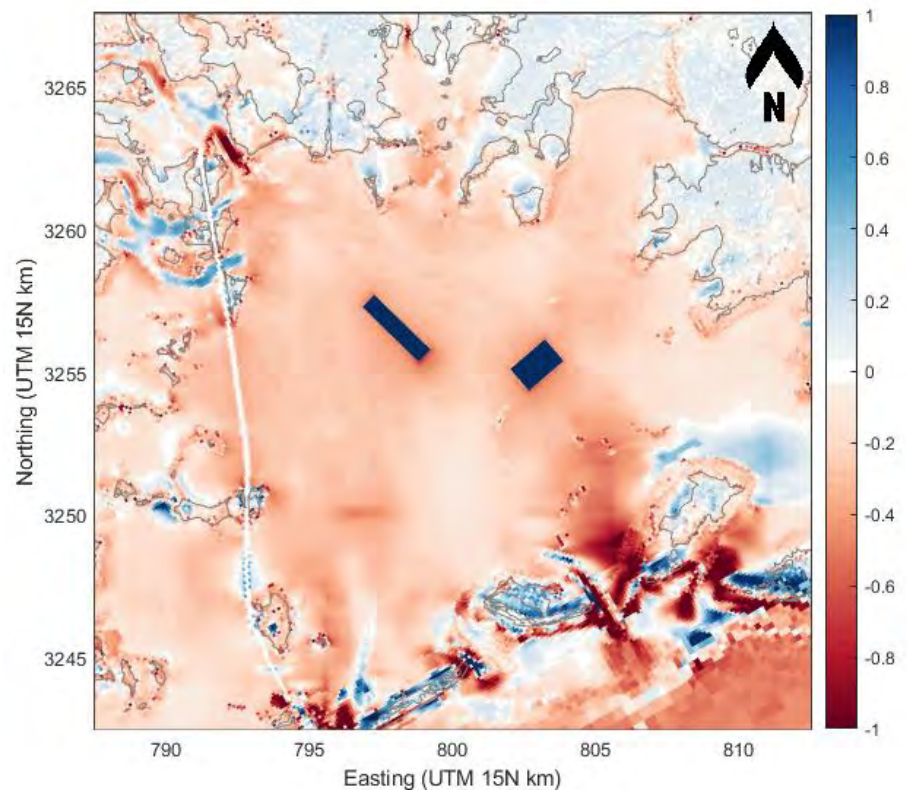
Figure B-20. Modeled bed level change (m) at Barataria Bay for S5 (BP1 in NW-SE orient. and BP2 in NE-SW orientation) after 10 years.
