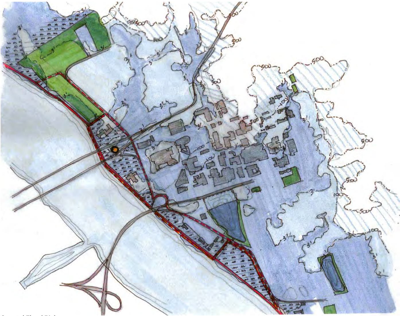
Coastal Flood Risk 100 and 500 Year Floodplain
