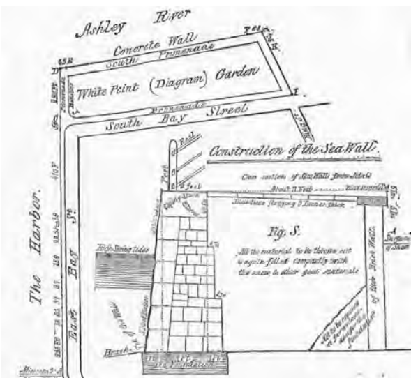
Fortification from the Sea High Battery plan and cross section. Image Credit: Parker Survey, 1855
