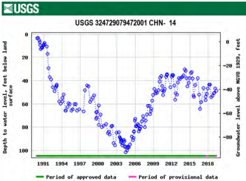
Figure 3 Groundwater Levels at observation well in downtown Charleston USGS
