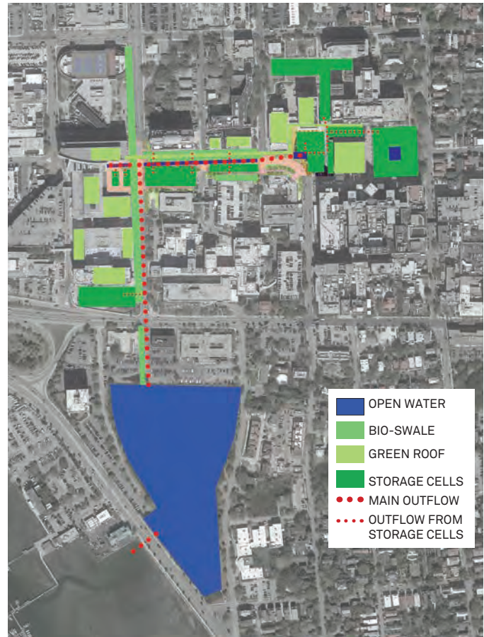
MUSC Facilities Master Plan Stormwater Strategy
