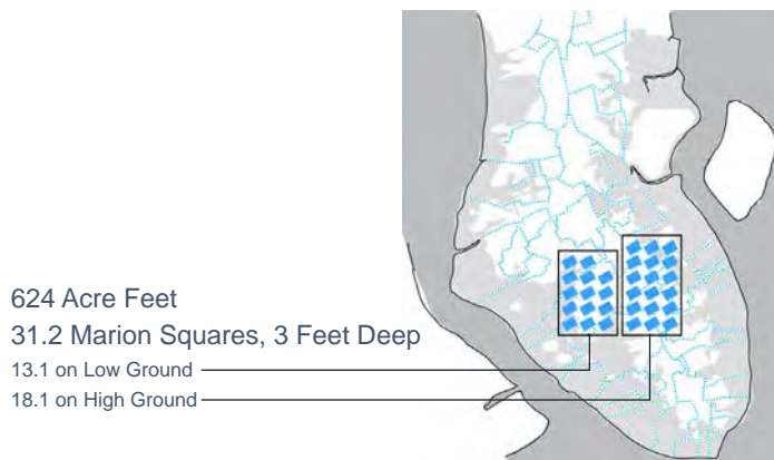
Water Assignment for a 25-Year (4% annual occurring chance) 1 Hour Storm Event
