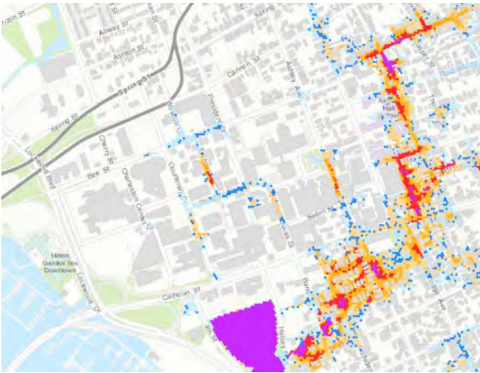
1 Year Storm Event Flooding Depth
