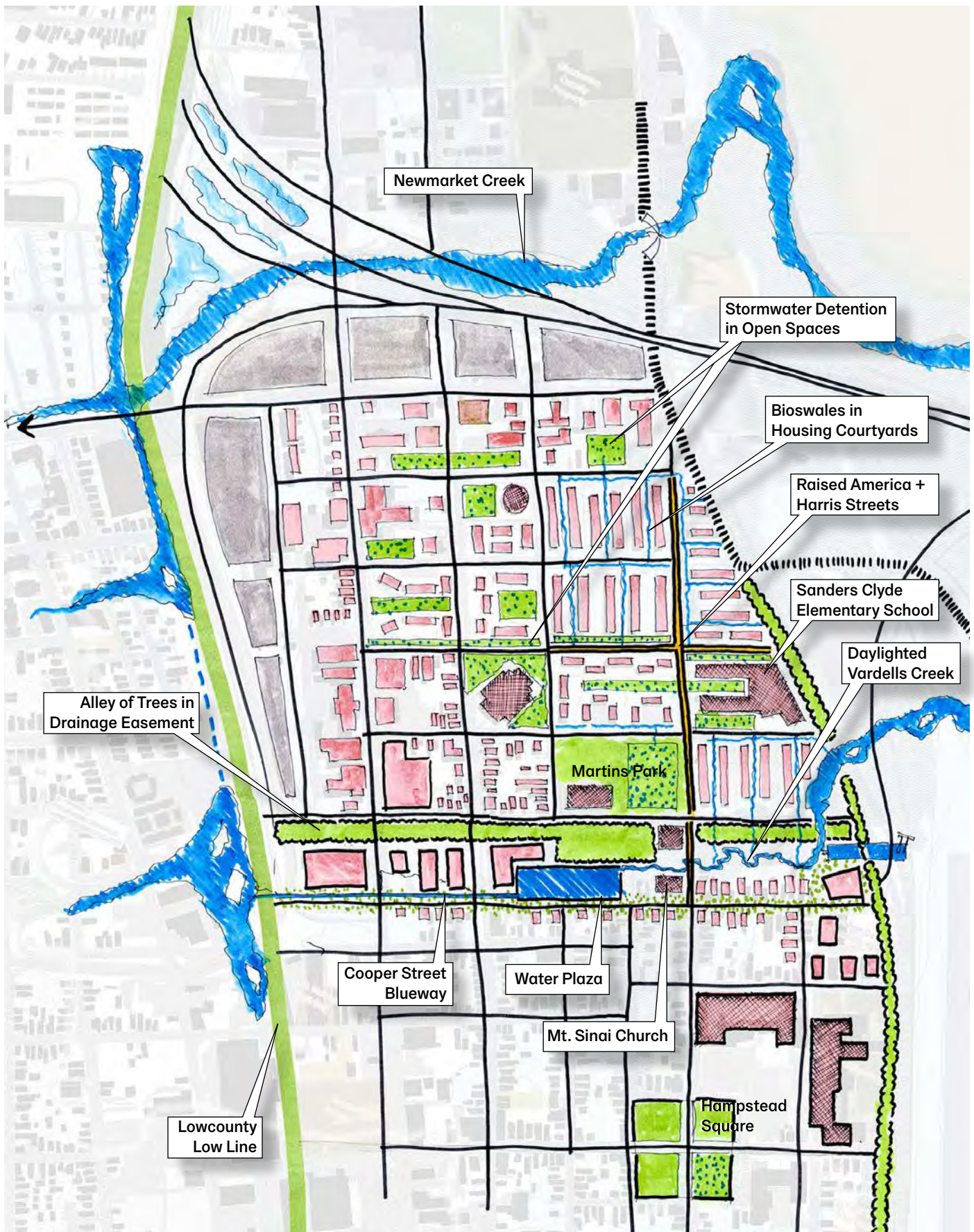
Enlarged Detail of Vision for Green Infrastructure and Elevated Roadways
