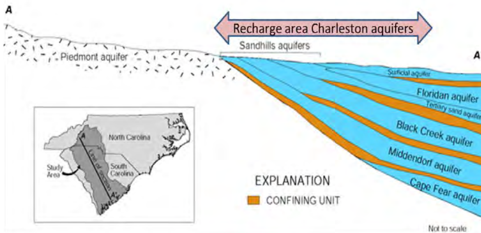
Figure 4 Regional Grounwater System
