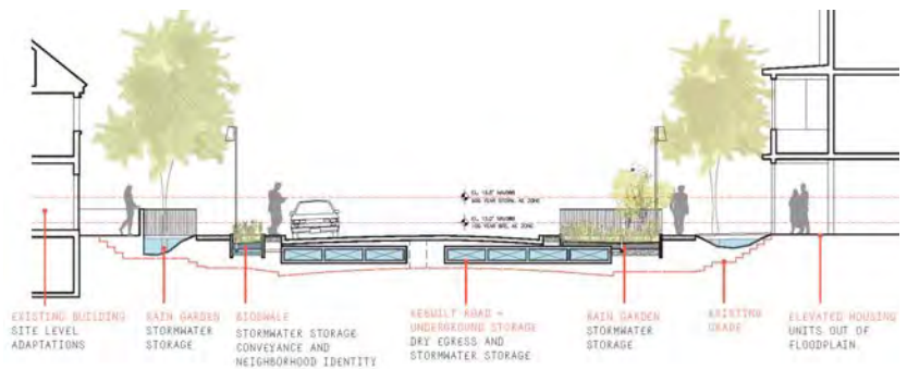
Raised Street Design for Bridgeport, CT Credit: Waggonner & Ball/YUDW, Resilient Bridgeport
