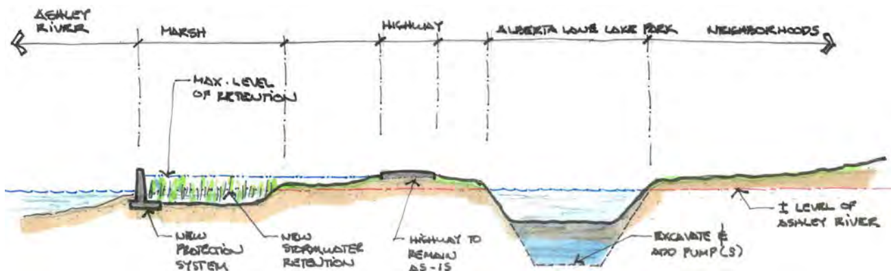
Section of Alignment B Perimeter protection encloses wetlands, increasing stormwater storage
