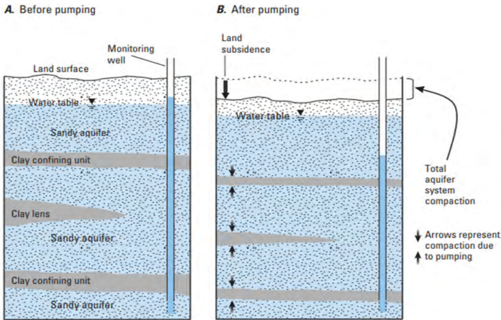
Figure 2 Aquifer-system compaction caused by groundwater withdrawals Modified from Galloway and others (1999)
