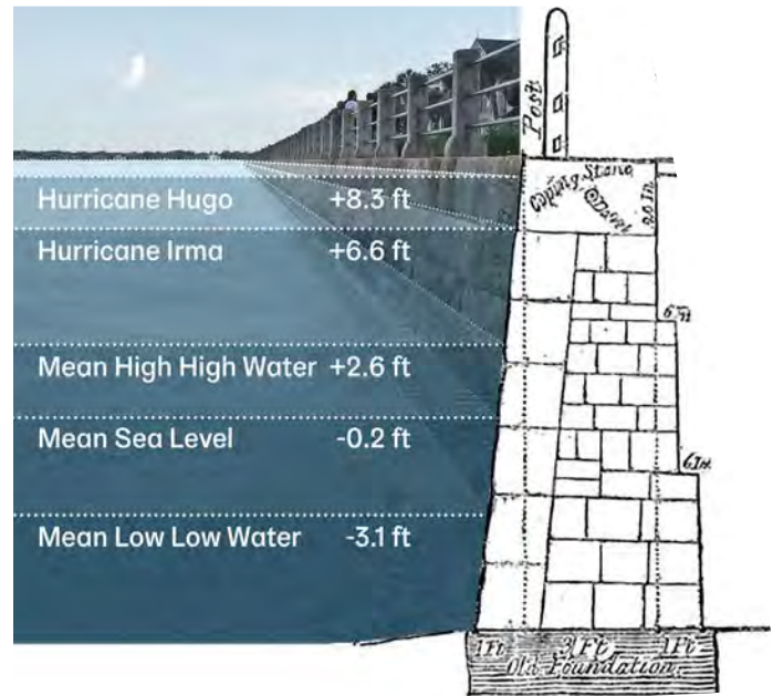
Tides & Storm Surge on the High Battery
