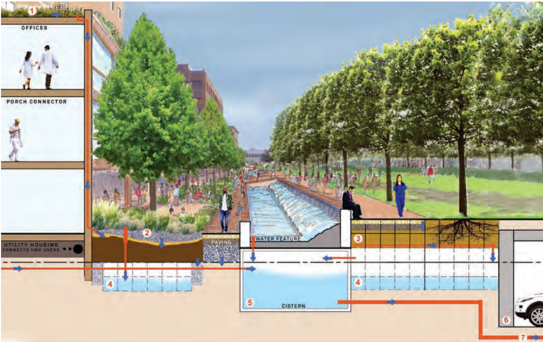
MUSC Facilities Master Plan Stormwater Strategy Credit: MUSC Master Plan
