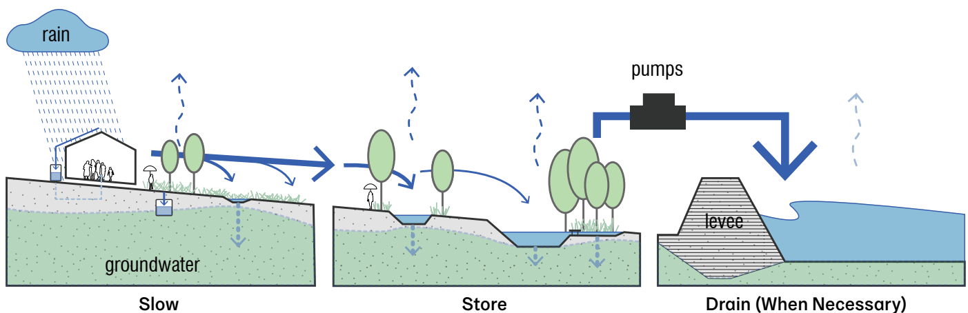
Slow-Store Approach to Stormwater Management
