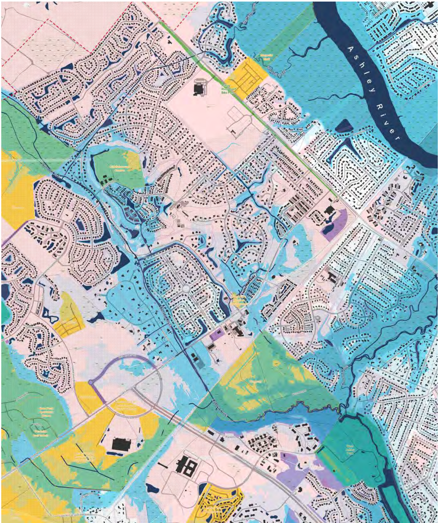
Floodplain and Development Floodplain is the light blue overlay and development sites are the yellow parcels
