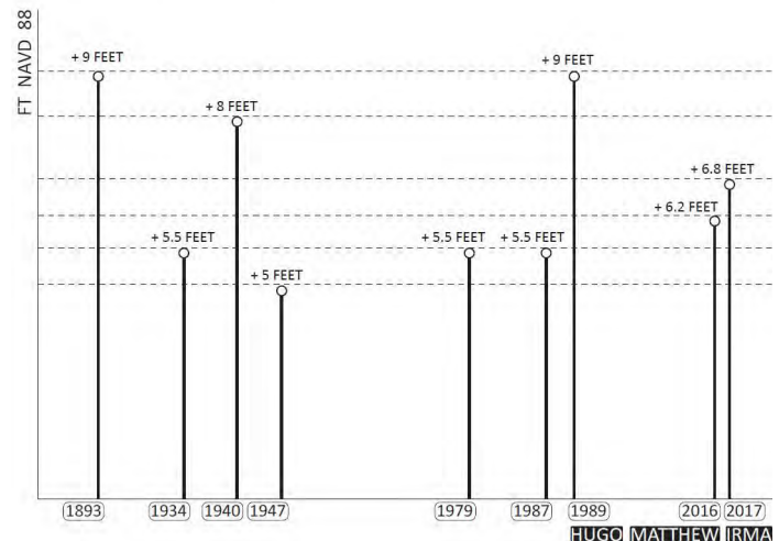
Historic Storm Surge High tide levels during historic storm events.
